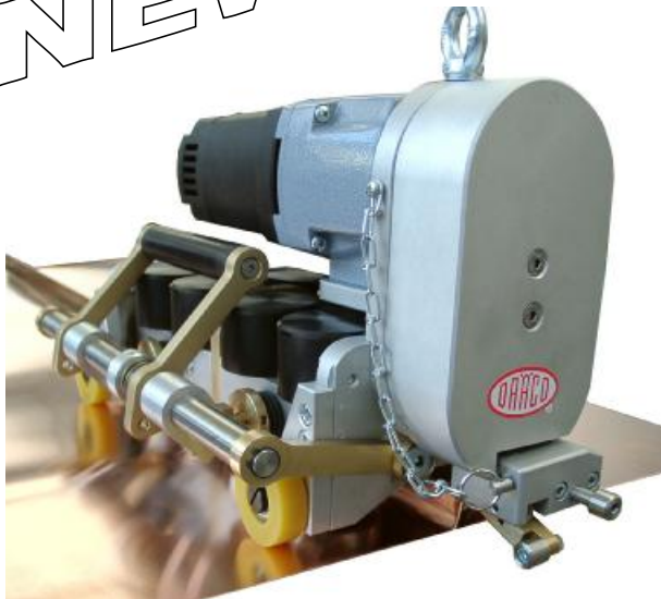
K9-1 with dual-safety switch K9-1-DF
